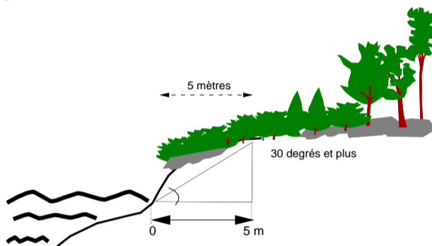
Figure 2.7d : Talus
